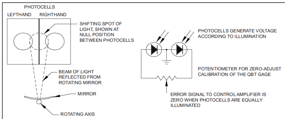
Figure 4. Photodiode Assembly.
